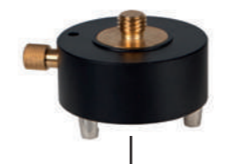
Ref.-No. 481 110-613 Leica-Style Prism Station, tribrach adapter with optical plummet. Accuracy: ± 2"
