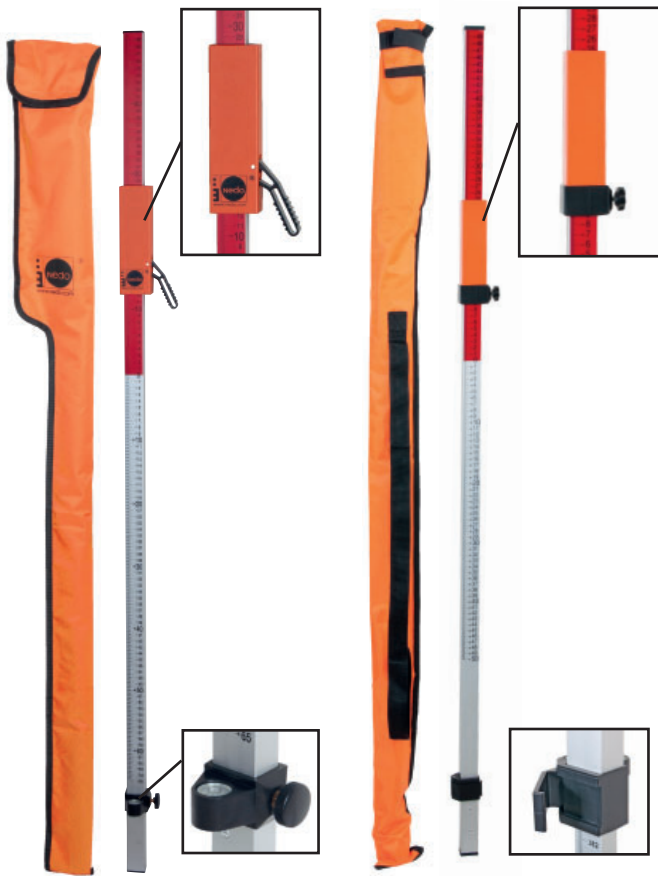
QualiLine Flexi Rod set Ref.-No. 360 916-622
